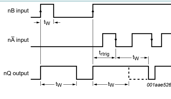
Fig. 12. Output pulse control using retrigger pulse n\overline{A}
