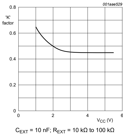
Fig. 10. Typical 'K' factor as a function of V_{CC}
