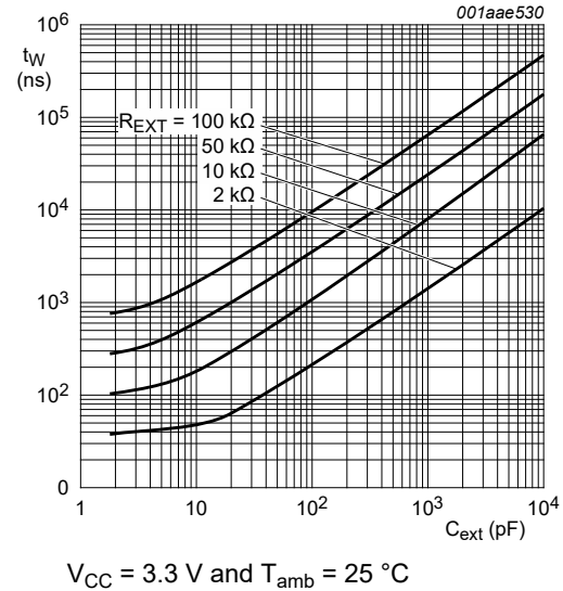
Fig. 11. Typical output pulse width as a function of the external capacitance values
